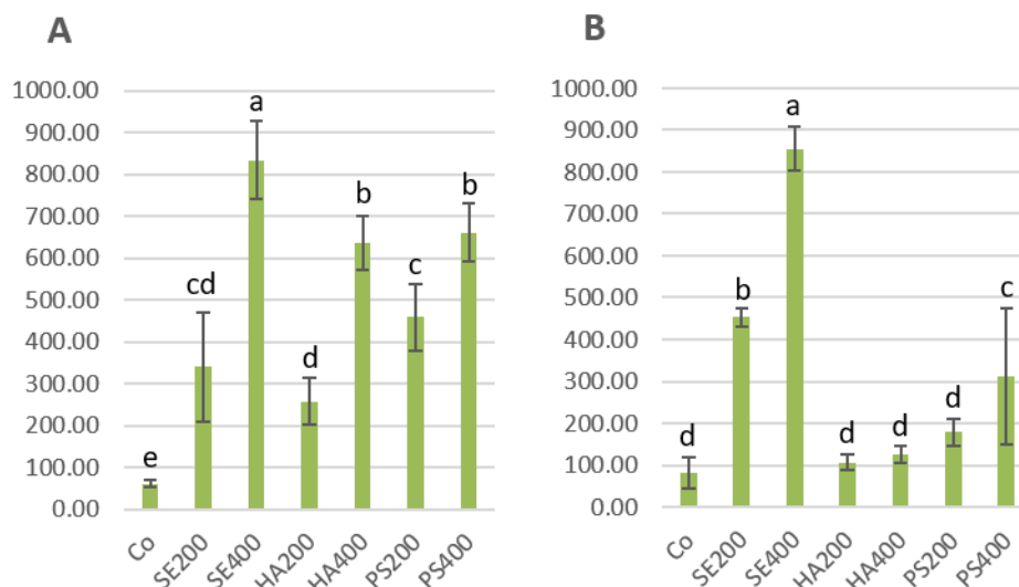
Figure 4. Selenium concentrations ( \mu\text{g/kg} ) in the edible part of the plant (leaf) per treatment in lamb's lettuce (A) and amaranth (B)
