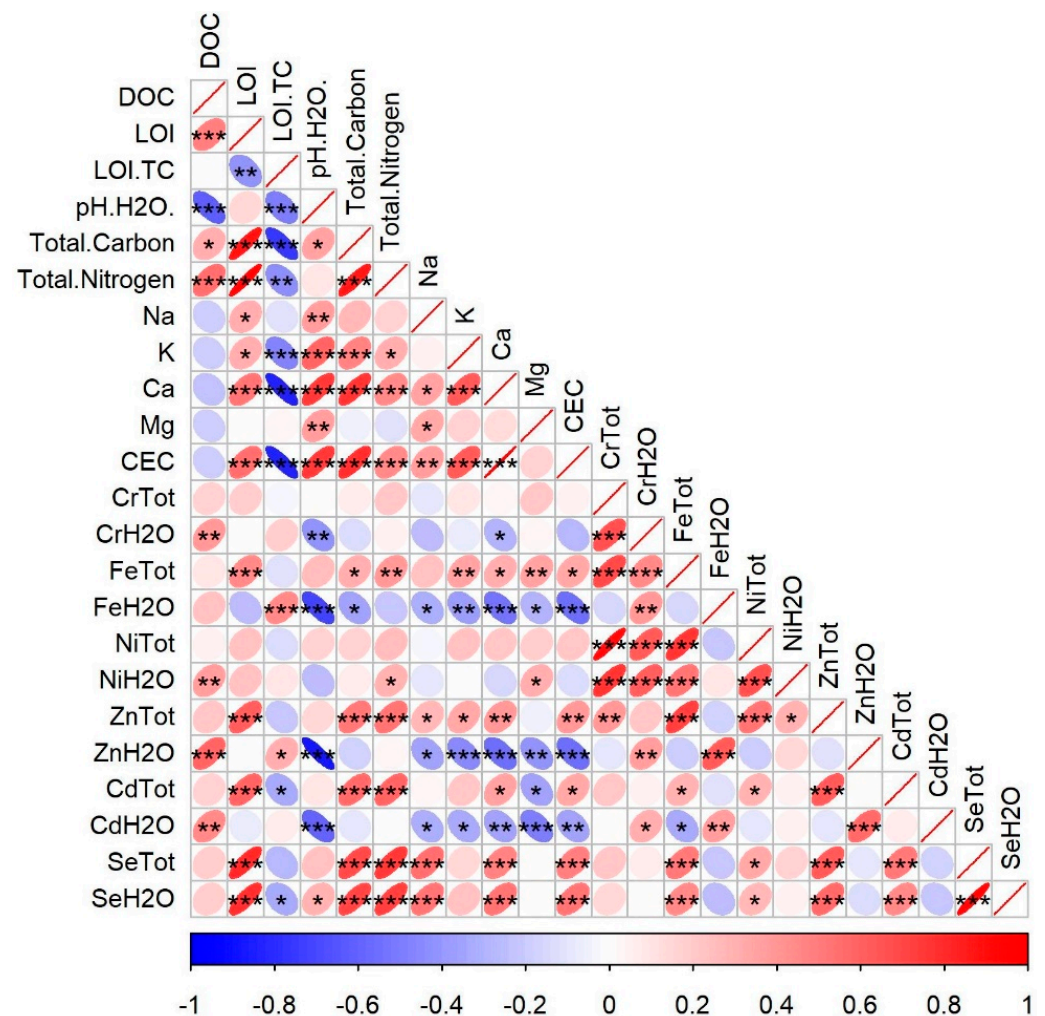
Figure 1. The illustration shows the negative (−, blue) and positive (+, red) correlations between soil properties and total soil and total water-extractable concentrations of several elements. Significance of correlation is denoted with * ( \alpha = 0.05 ), ** ( \alpha = 0.01 ), and *** ( \alpha = 0.001 ).
